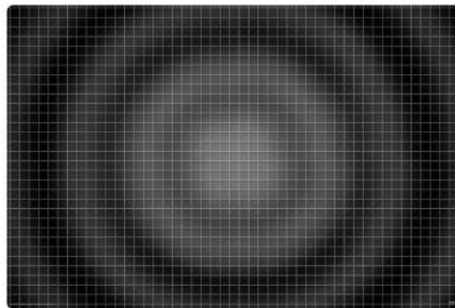
DS007 Graphite
